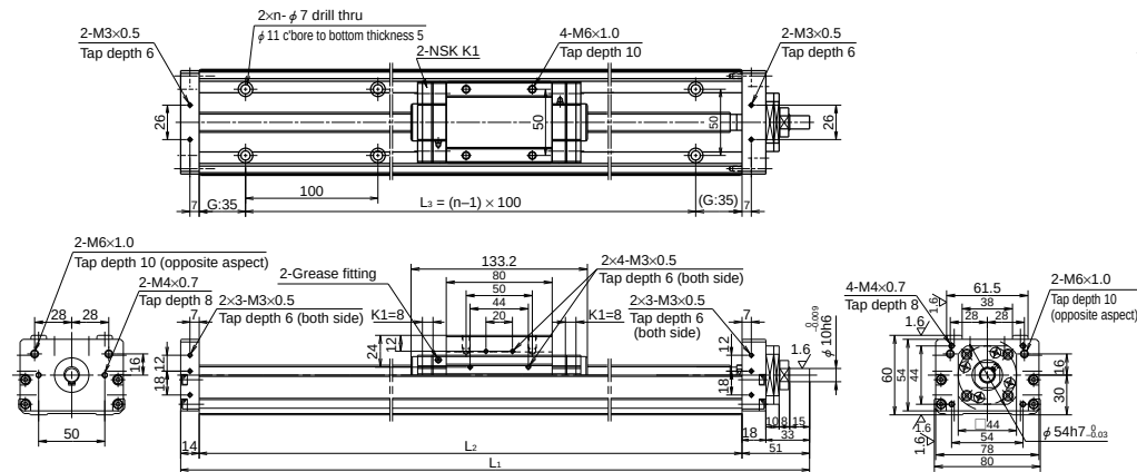
Dimension of MCM08 (Single Slider)
