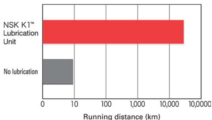
Results of High-Speed Durability Test of Ball Screws Without Lubricant
