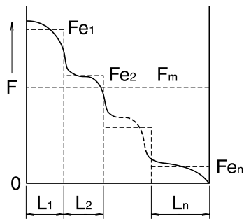
Stepwise Fluctuating Load
