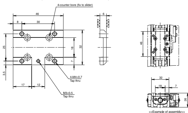
MC-SP03-00 (for Ball Screw Lead 1 and 2 mm)
