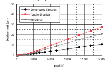
TCH10 short slider
