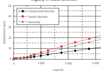
TCH09 short slider
