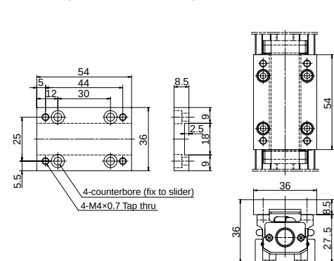
MC-SP03-01 (for Ball Screw Lead 15mm)
