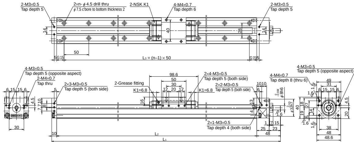
Dimension of MCM05 (Single Slider)
