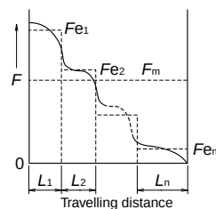
Stepwise Fluctuating Load
